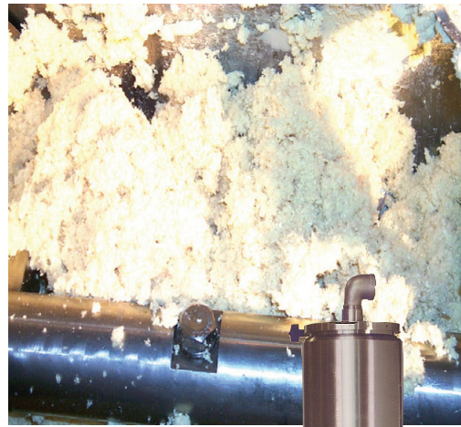
Closeup of Aramid Fiber after opening in Processall Mixer
